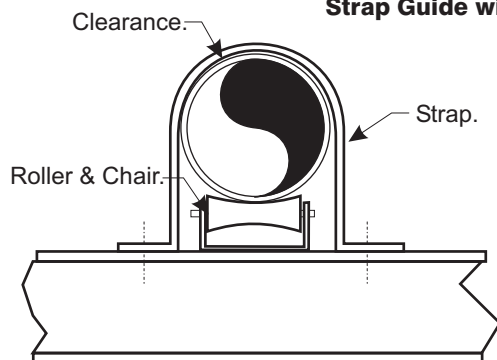
Strap Guide with Roller & Chair.
