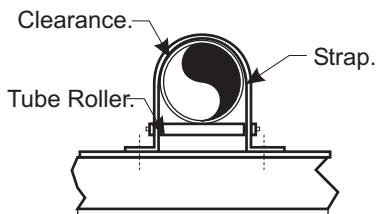
Strap Guide with Tube Roller.
