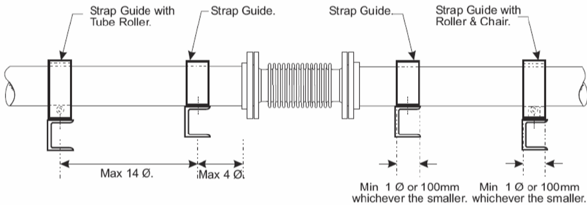
Strap Guide with Roller & Chair.
