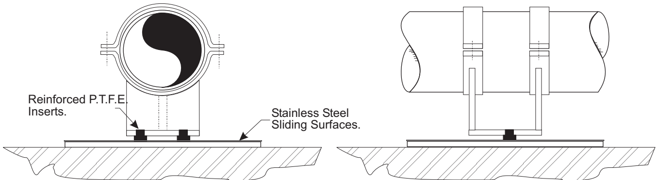
Heavy Duty Skid Guide.
