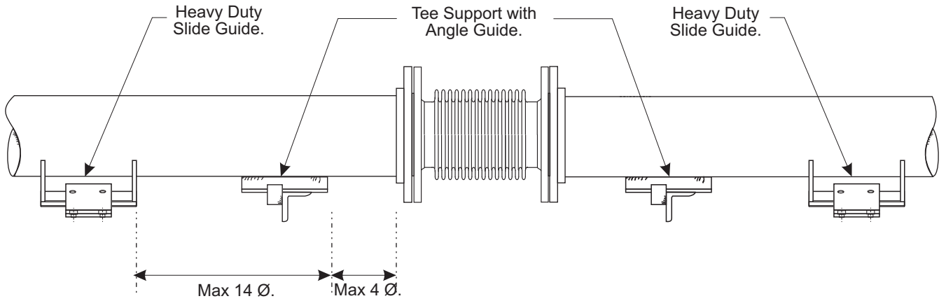
Tee Support with Angle Guide.
