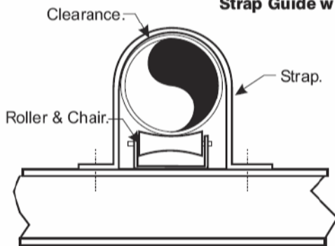
Strap Guide with Roller & Chair.
