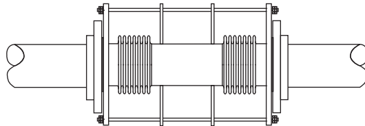
Flanged Type JP120.
