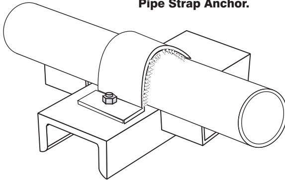
Pipe Strap Anchor.
